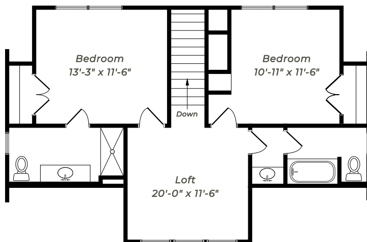
UPPER LEVEL
